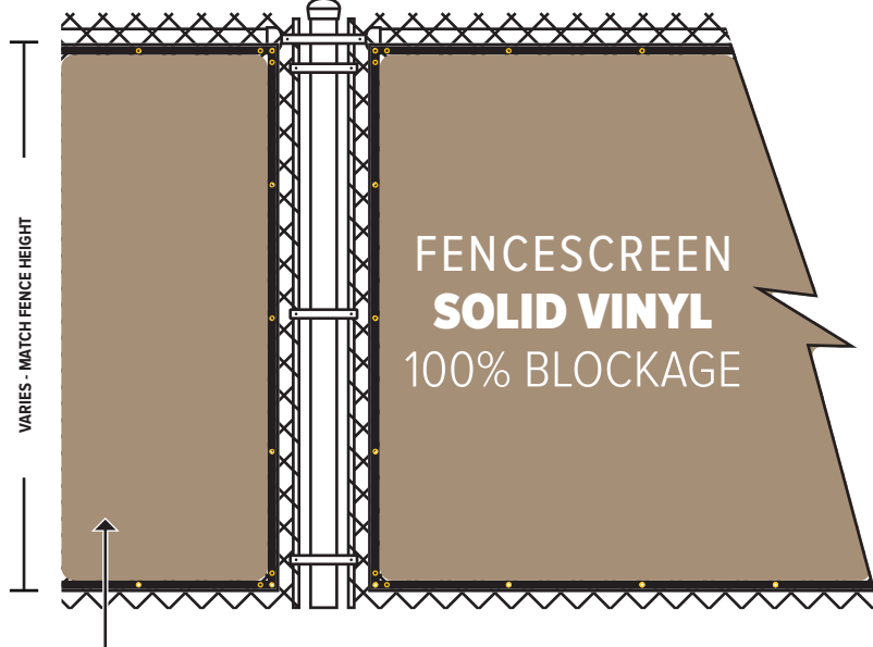
ELEVATION VIEW
